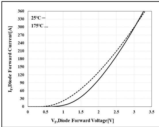
Figure 15.Diode Forward Characteristics
