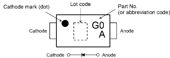
Fig. 7.1 Marking
