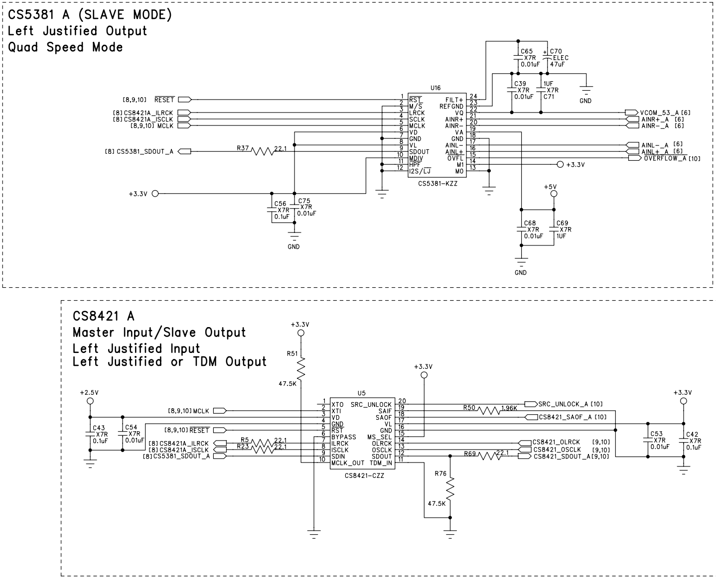
Figure 11. CS5381 & CS8421 Pair A
