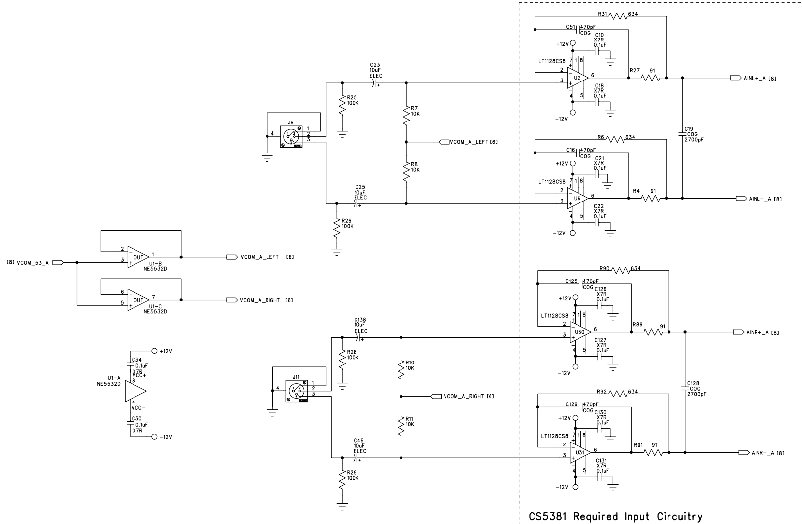
Figure 9. Analog Inputs 1 & 2
