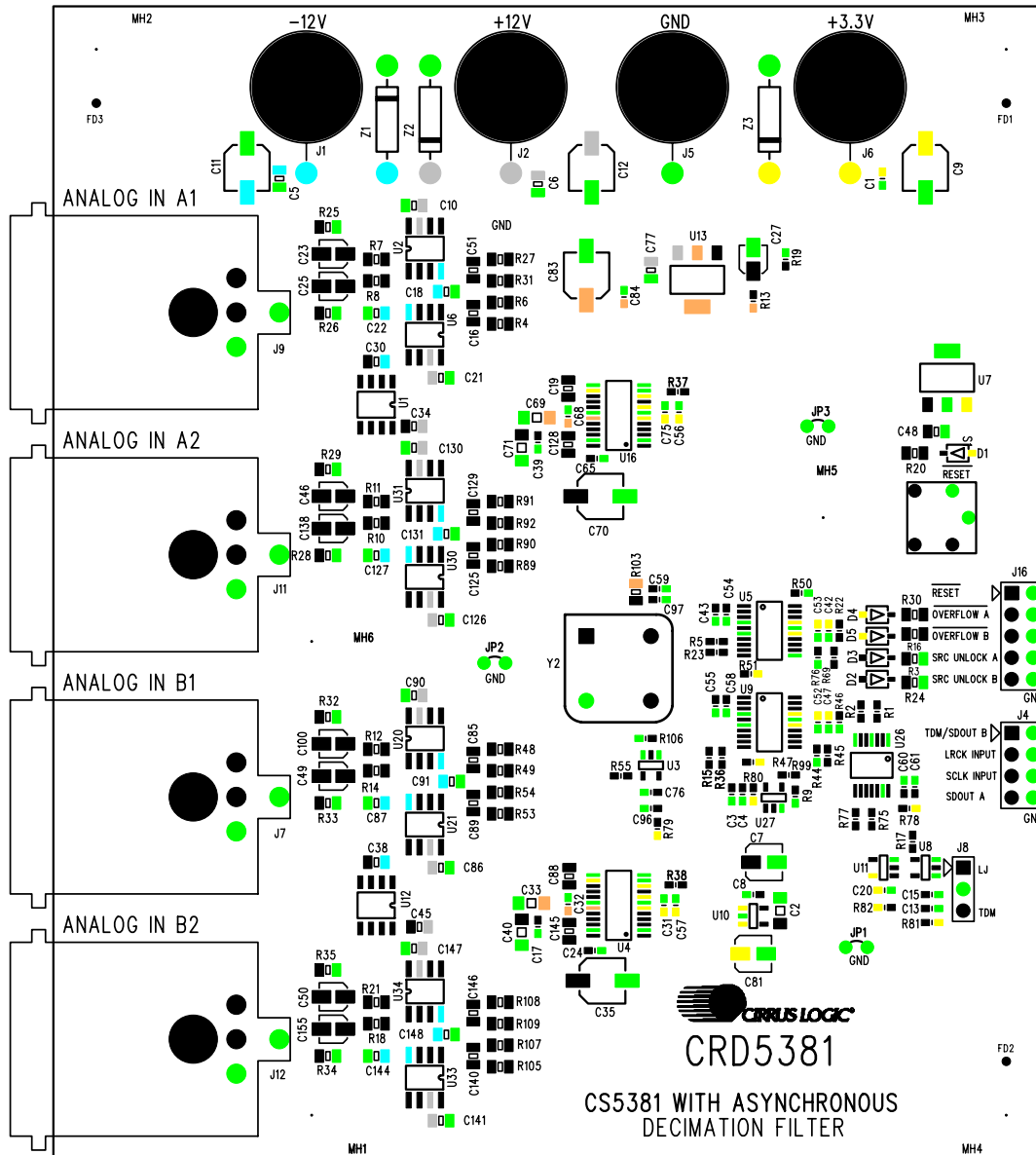
Figure 15. Silk Screen
