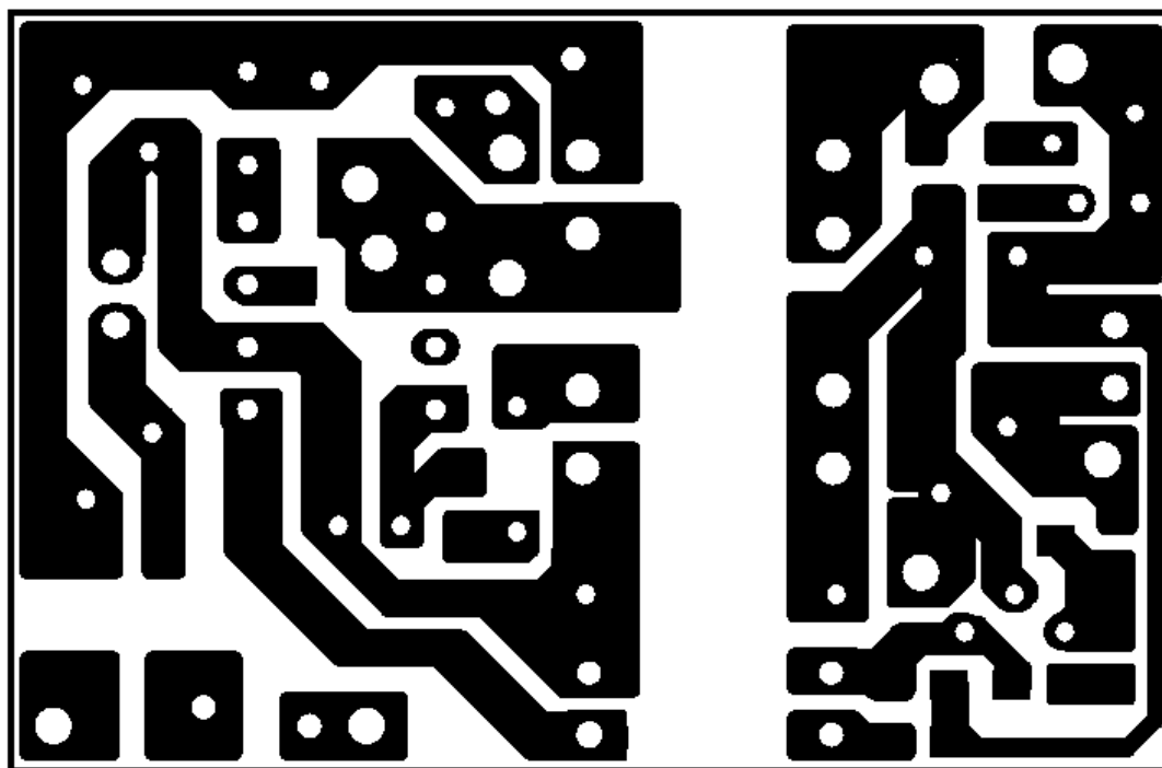
PCB Layout
