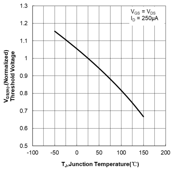
Figure.10 Typical Theshold Voltage vs Junction Temperatu
