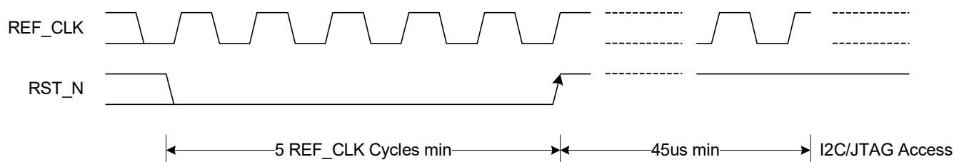
Figure 23: Reset Timing
