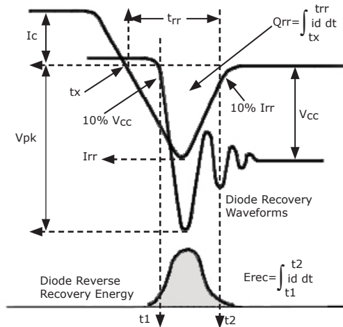
Fig 12. Body Diode Recovery Waveform
