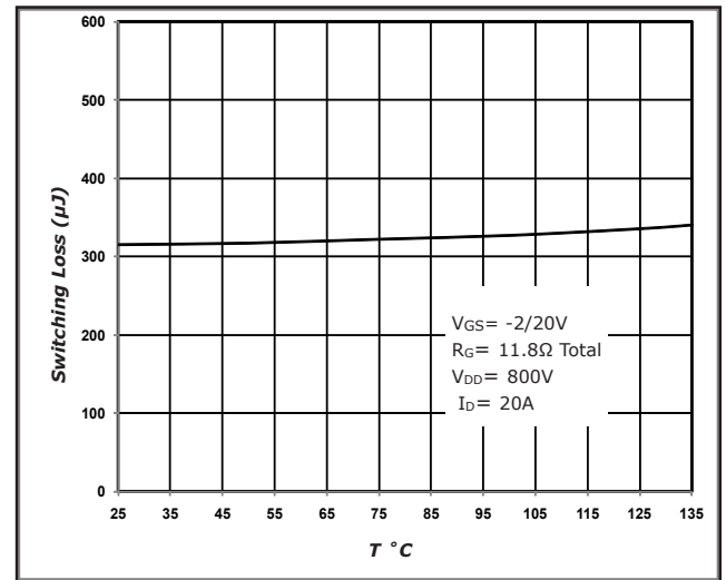
Fig 7. Inductive Switching Energy(Turn-off) vs. T
