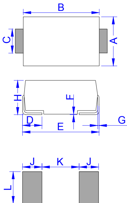
DO-214AA (SMB)
