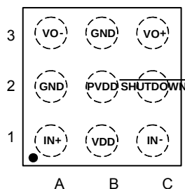
CSP9 Package ( Top View )
