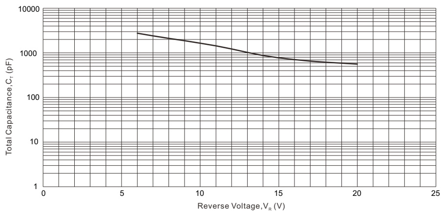
Fig. 5 - Total Capacitance VS. Reverse Voltage
