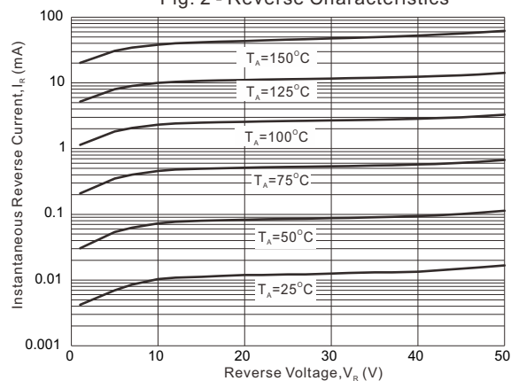
Fig. 2 - Reverse Characteristics
