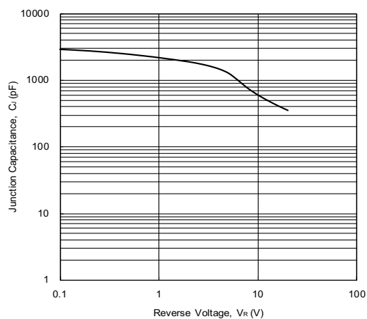
Fig. 5 - Junction Capacitance
