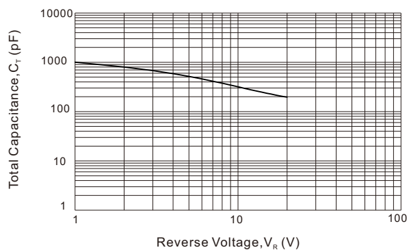
Fig. 3 - Total Capacitance VS. Reverse Voltage (per diode)
