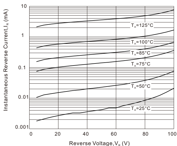
Fig. 2 - Reverse Characteristics (per diode)
