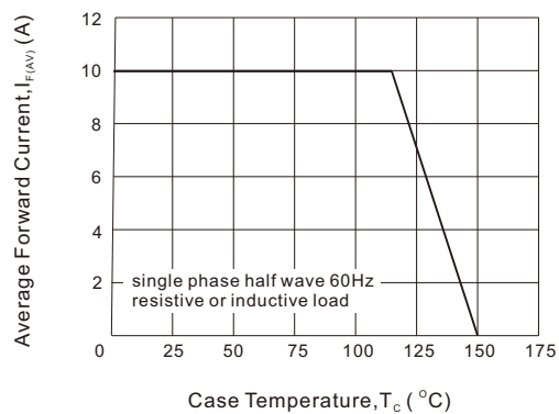
Fig. 4 - Forward Current Derating Curve
