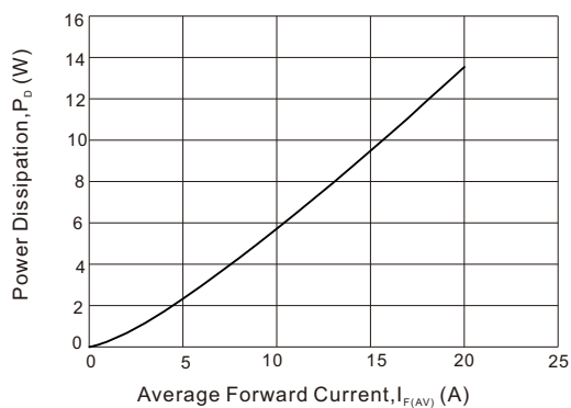
Fig. 5 - Forward Power Dissipation (per diode)
