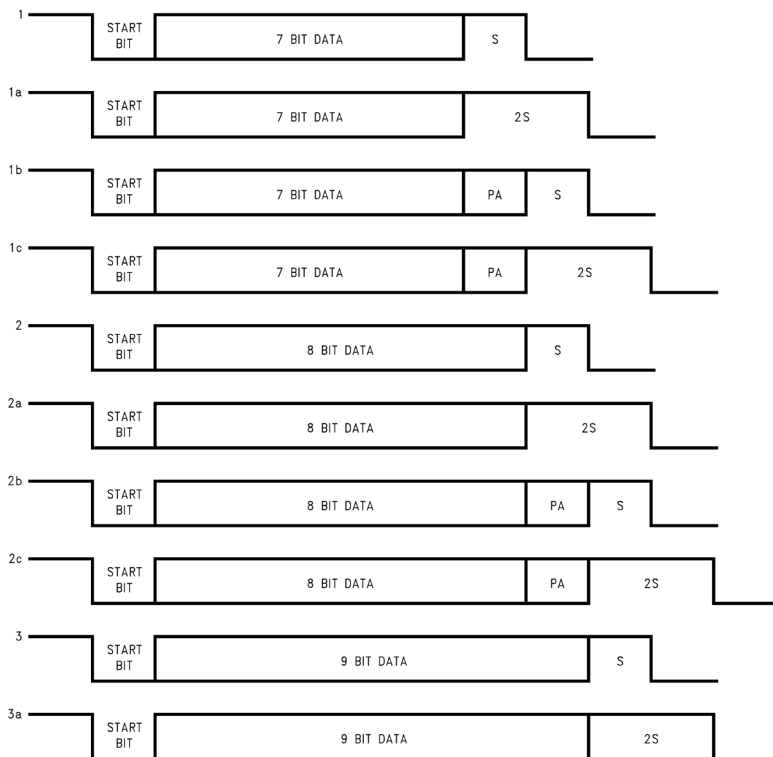
FIGURE 23. Framing Formats
