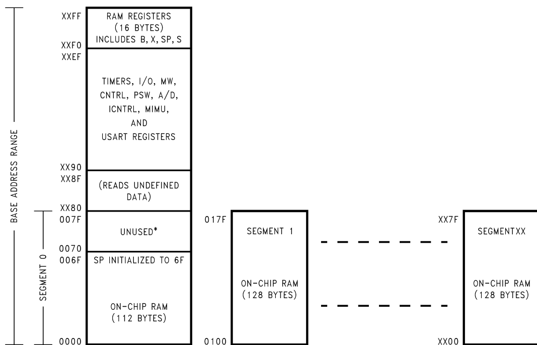
FIGURE 7. RAM Organization
