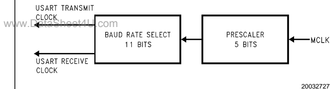
FIGURE 24. USART BAUD Clock Generation
