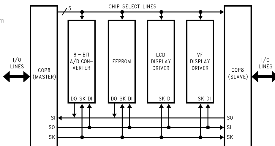
FIGURE 29. MICROWIRE/PLUS Application
