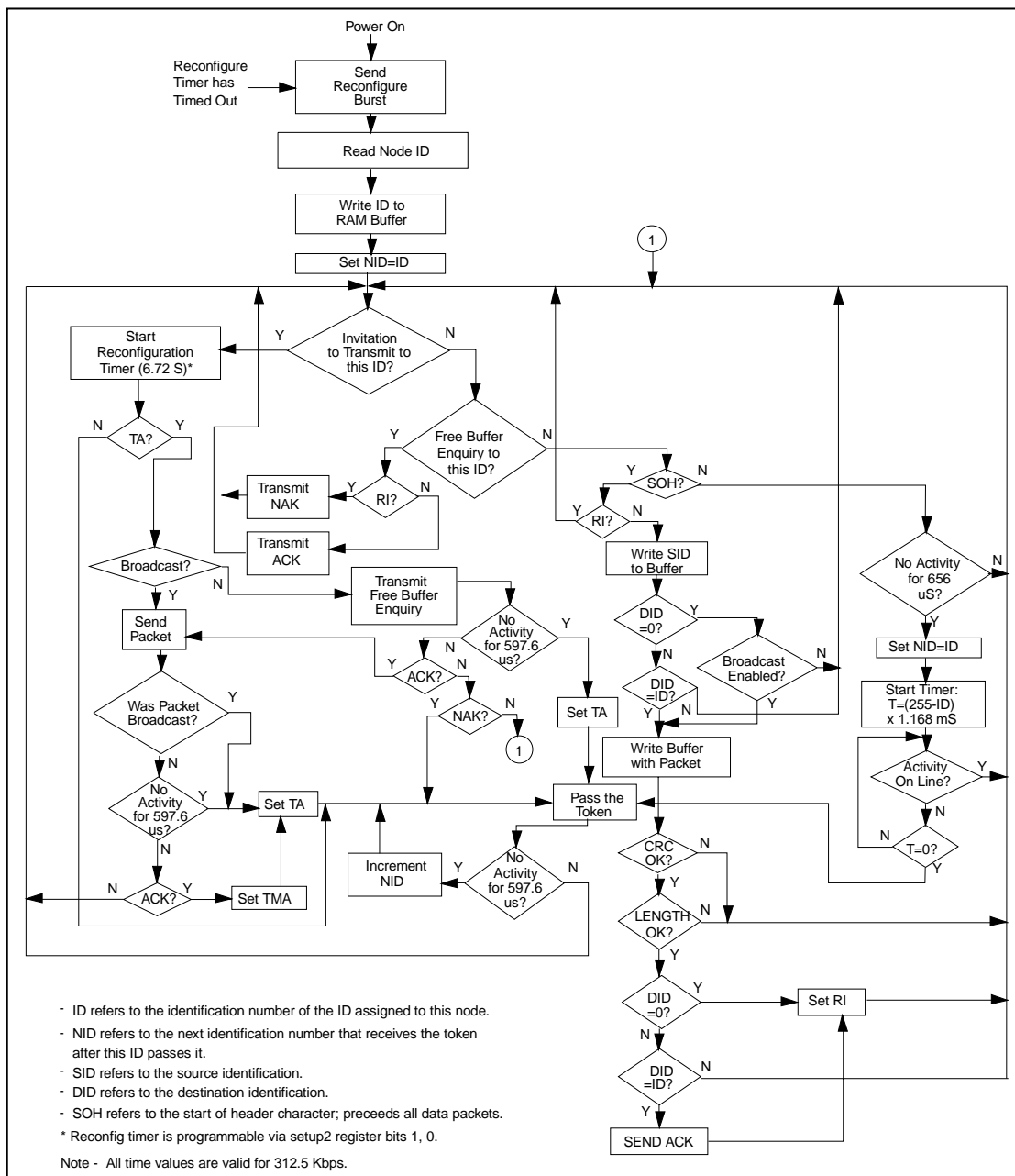
Figure 3.1 - COM20019I OPERATION
