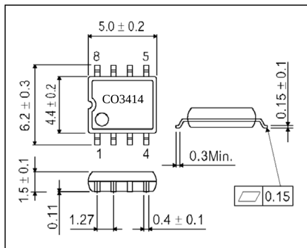
SOP-8
