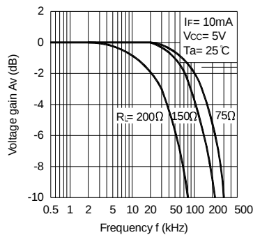
Fig.11 Frequency Response
