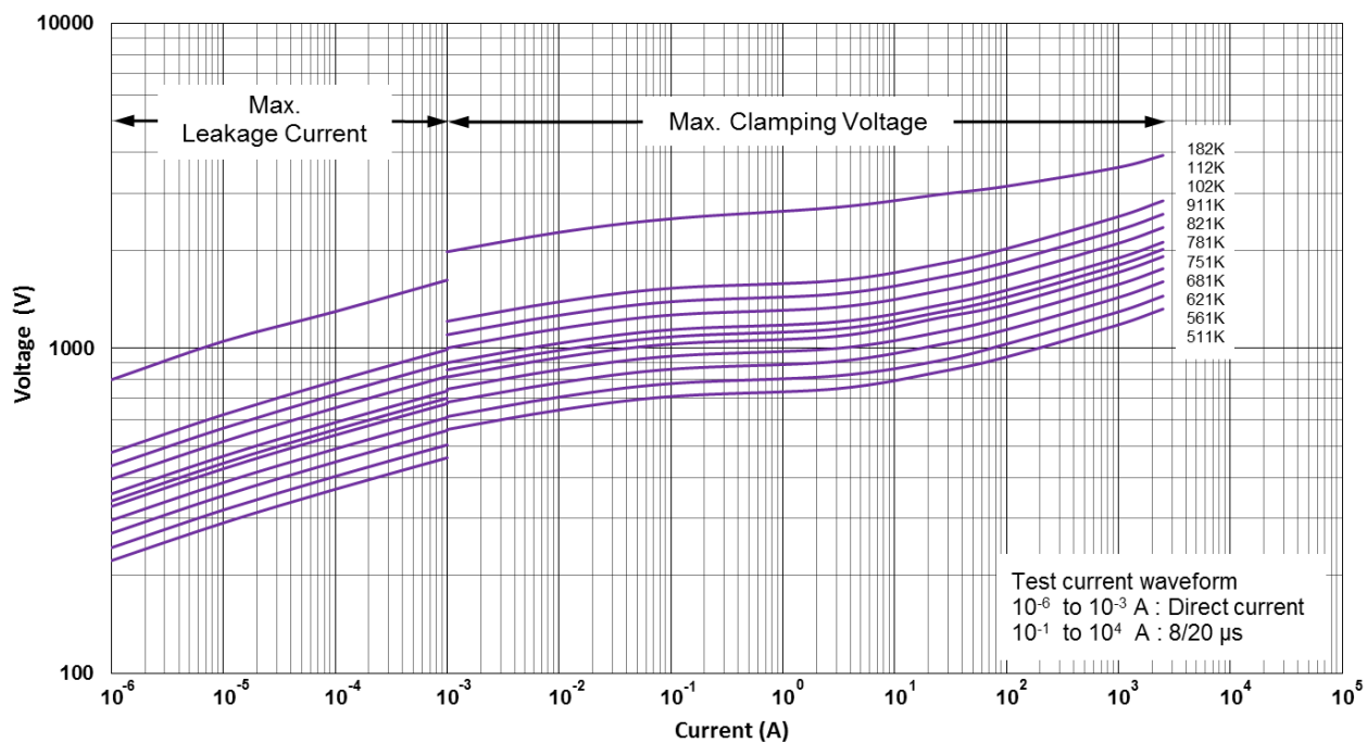
CNR-10D511K to CNR-10D182K V-I Curves
