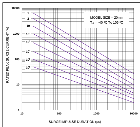
CNR-20D820K to CNR-20D751K
