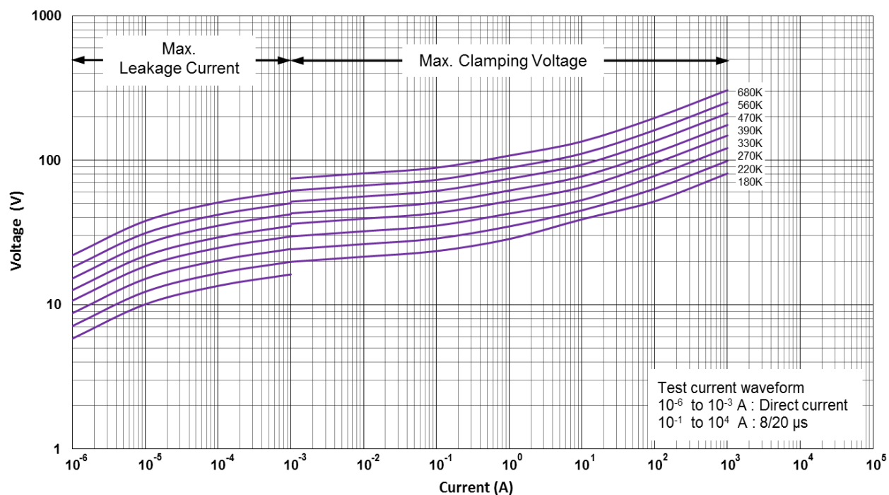
CNR-14D180K to CNR-14D680K V-I Curves
