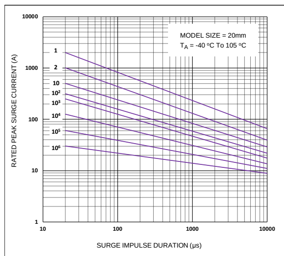
CNR-20D180K to CNR-20D680K
