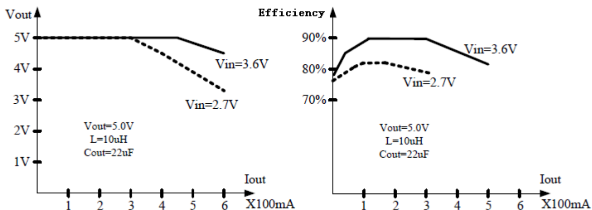
Figure 3 Operating Profile
