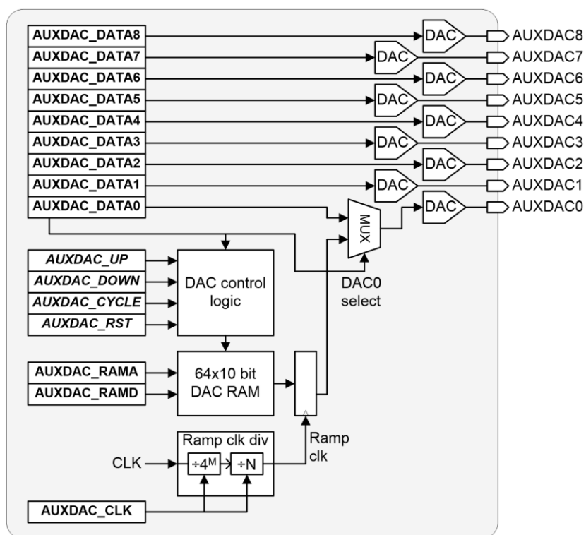
Figure 28 Auxiliary DACs
