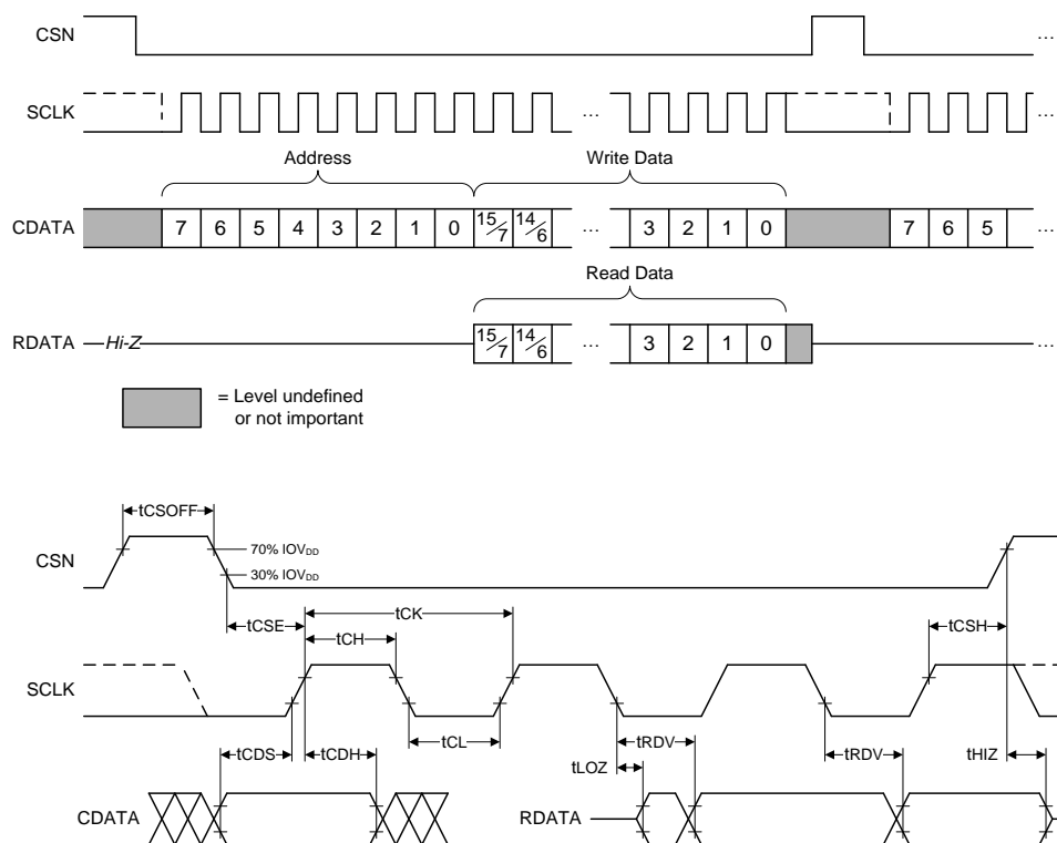
Figure 31 C-BUS Timings
