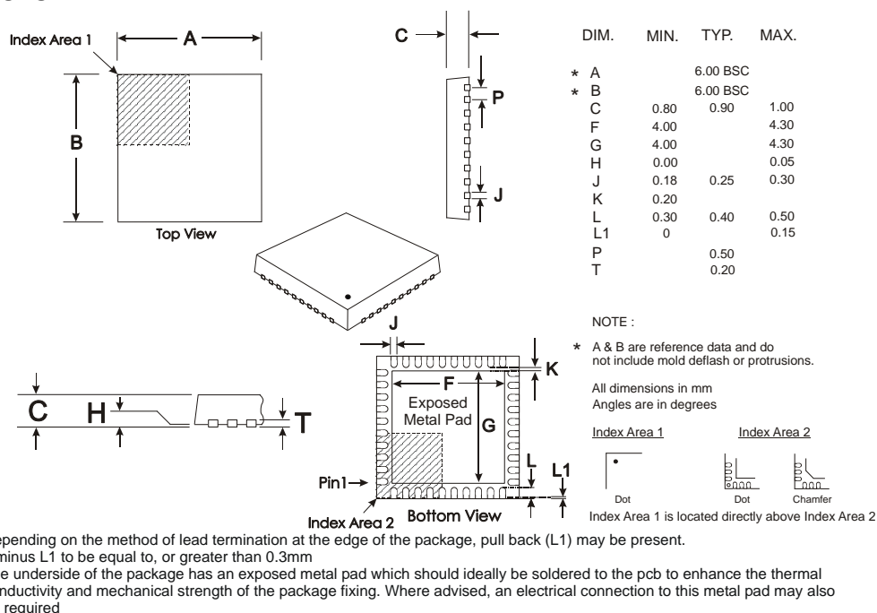
Figure 22 Q4 Mechanical Outline
