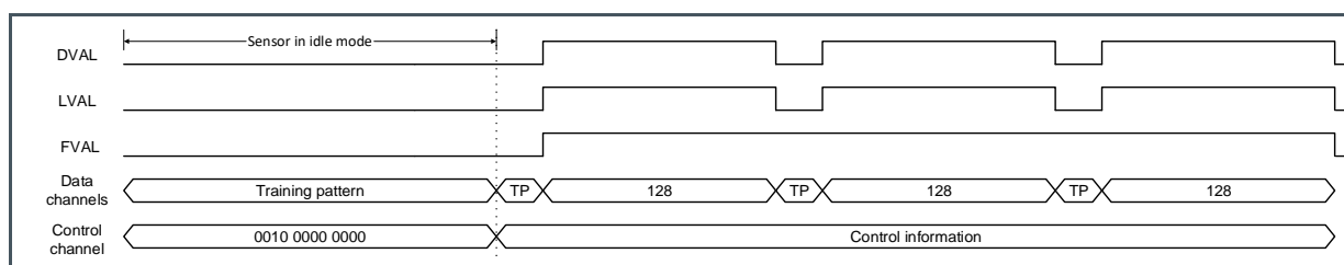
Figure 52: Training Pattern Location in the Data and Control Channels.
