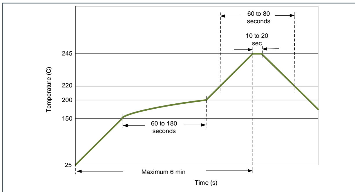
Figure 104: Reflow Soldering Graph
