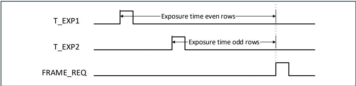
Figure 56: Interleaved Read-Out in External Exposure Mode
