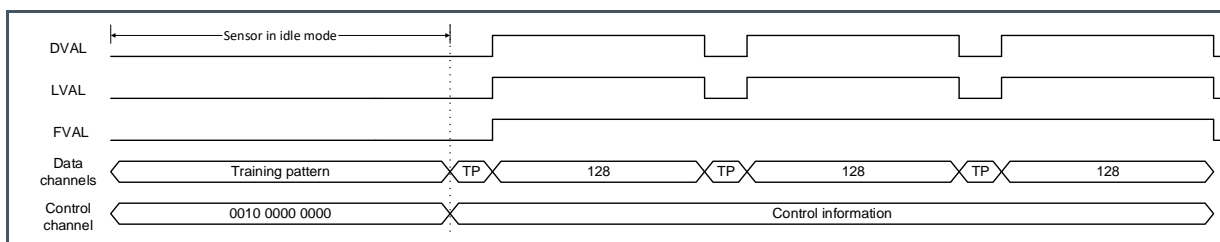
Figure 76: Training Pattern Location in the Data and Control Channels
