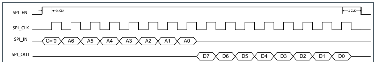
Figure 27: SPI Read Timing
