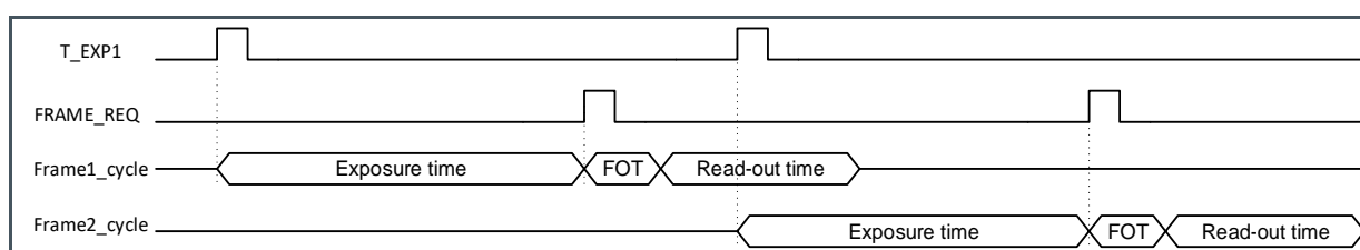
Figure 33: Request for 2 Frames Using External-Exposure-Time Mode
