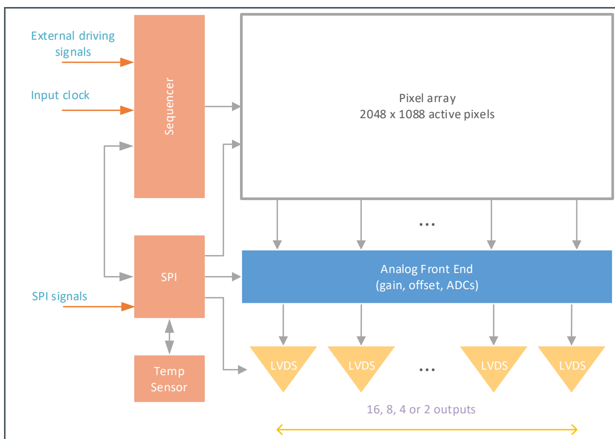
Figure 2 : Functional Blocks of CMV2000
