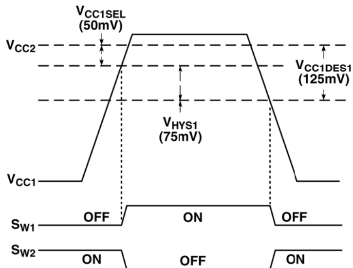
Figure 1. Supply Threshold Diagram (Hysteresis Input Pin Floating, See Typical Application Circuit, Page 2)
