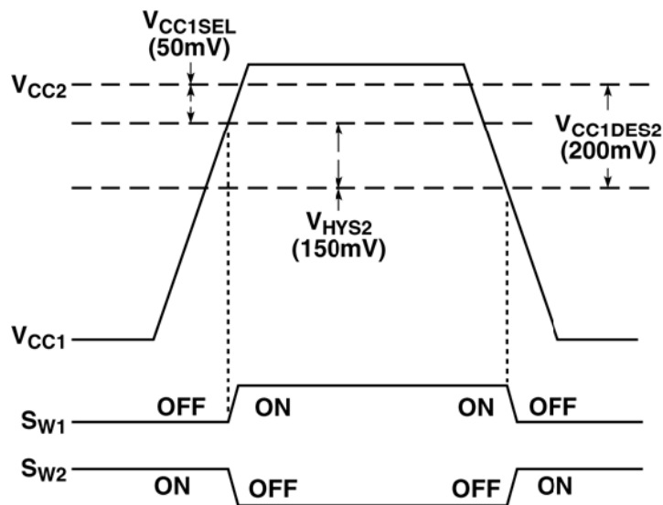
Figure 2. Supply Threshold Diagram (Hysteresis Input Tied to Ground, See Typical Application Circuit, Page 2)
