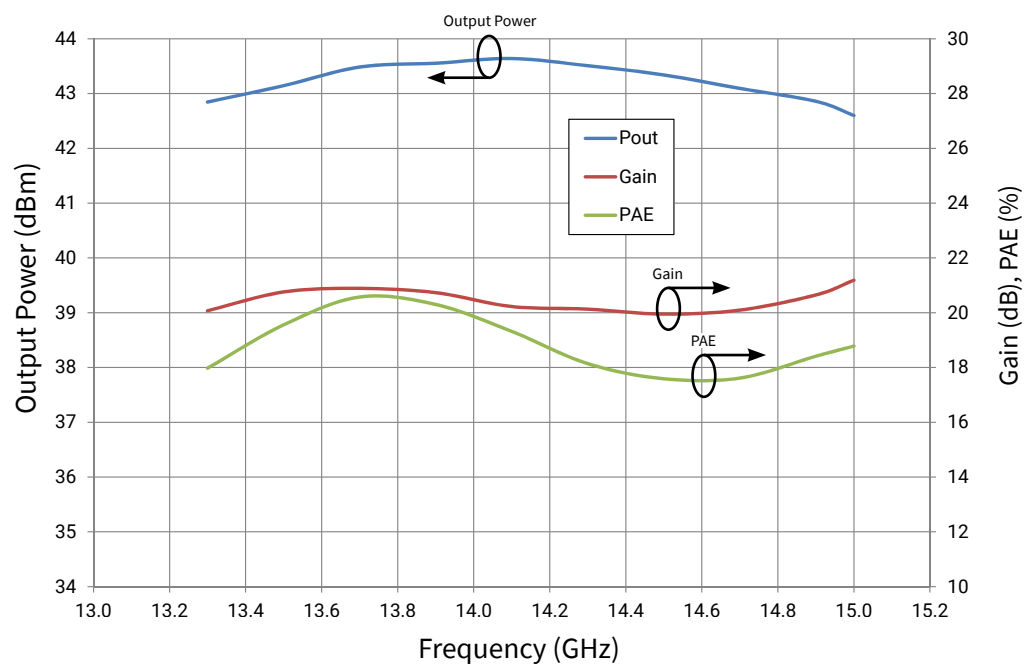
Figure 2. Modulated @ Spectral Regrowth = -30dBc, 1.6 MHz from Carrier 1.6 Msps OQPSK Modulation
