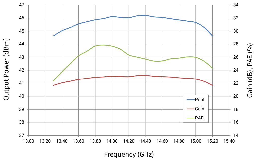
Figure 12. Pulsed vs. Frequency @ PIN = 23 dBm CMPA1D1E025F in Test Fixture V_{DD} = 40\text{ V} , I_{DQ} = 240\text{ mA} , 100 \mu\text{s} Pulse Width, 10% Duty Cycle, T_{case} = 25^{\circ}C
