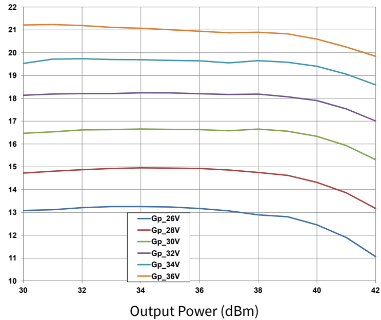
Figure 17. CMPA1D1E025F Modulated Power Sweep (Gp) 1.6 Msps OQPSK Modulation, Frequency = 14 GHz V_{DD} = 26\text{-}36\text{ V} , I_{DQ} = 150\text{ mA} , T_{case} = 25^\circ\text{C}
