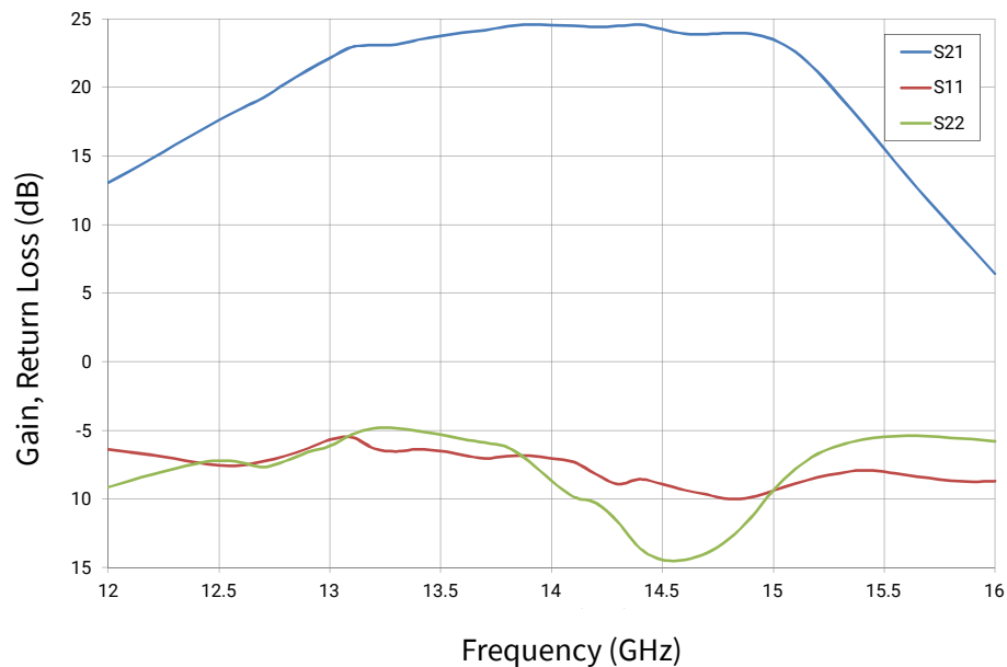
Figure 1. Small Signal S-Parameters CMPA1D1E025F in Test Fixture
