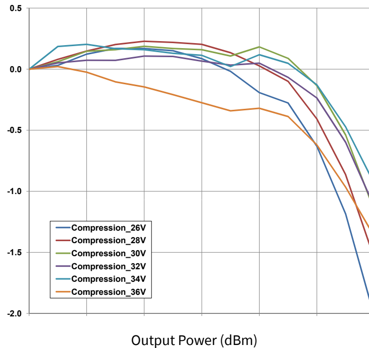
Figure 18. CMPA1D1E025F Modulated Power Sweep (Gain Compression) 1.6 Msps OQPSK Modulation, Frequency = 14 GHz V_{DD} = 26\text{-}36\text{ V} , I_{DQ} = 150\text{ mA} , T_{case} = 25^\circ\text{C}
