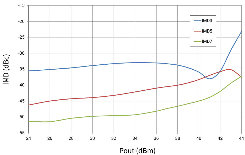
Figure 8. Two Tone Power Sweep IMD @ 1 MHz Carrier Spacing, 14 GHz
