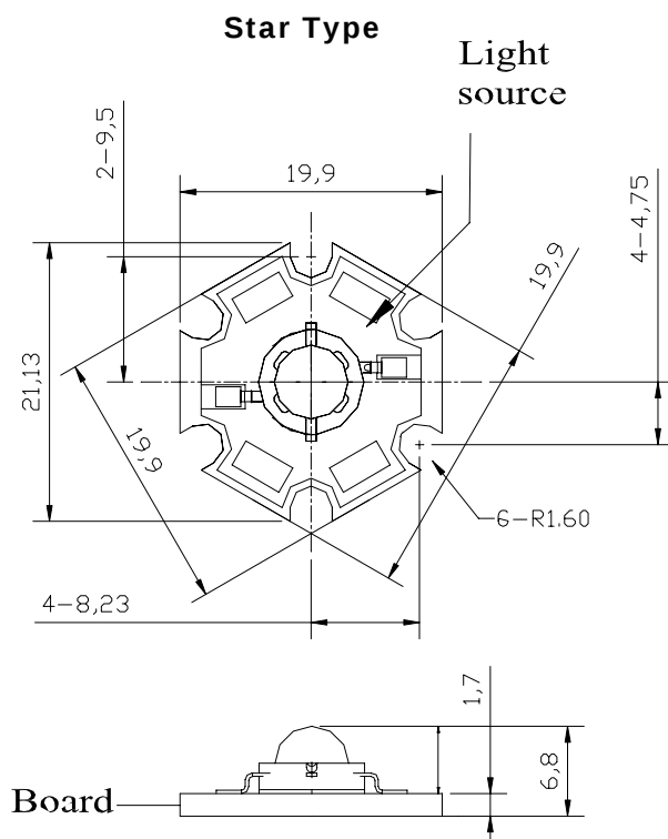
CMDA49xx15D13L Star Configuration
