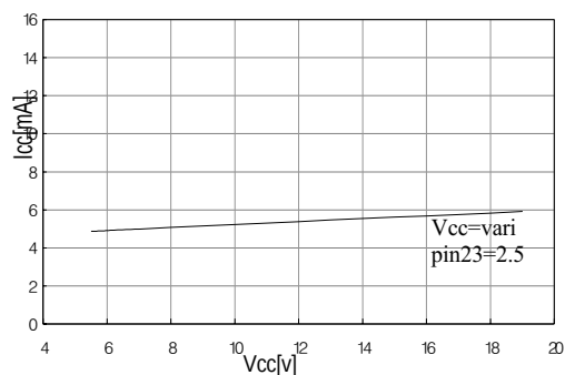
Figure 1. VCC vs. ICC
