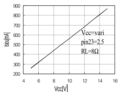
Figure 3. VCC vs. ISOU
