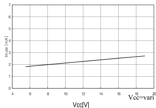
Figure 2. VCC vs. Imute
