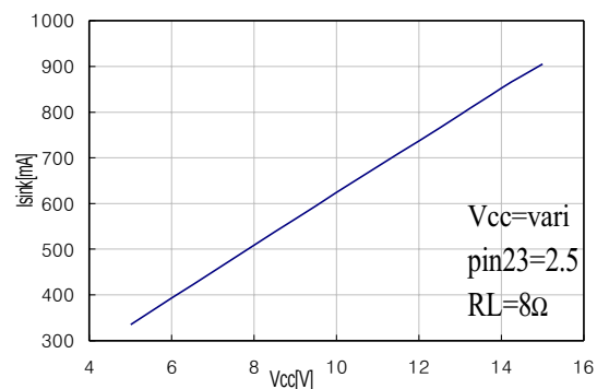
Figure 4. VCC vs. ISink
