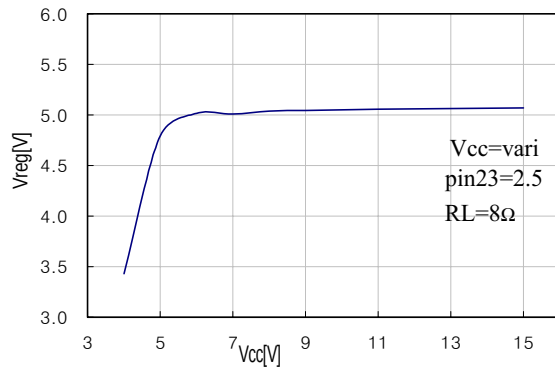
Figure 7. VCC vs. Vreg
