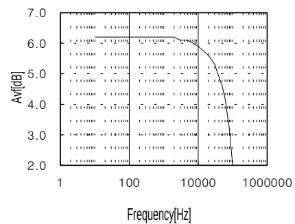
Figure 8. Frequency vs. Avf
