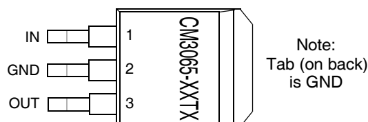
3-lead TO-263
