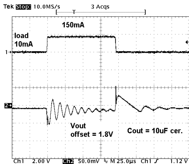
Figure 2. "Marginal" load transient response 1.8V output with 10 \mu F ceramic capacitor
