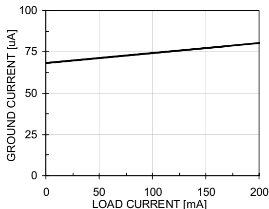
Ground Current vs. Load (VIN = 3.8V)
