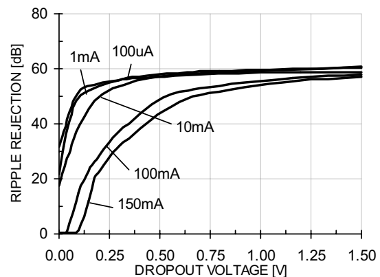
Power Supply Ripple Rejection Vs. Voltage Drop (1kHz)
