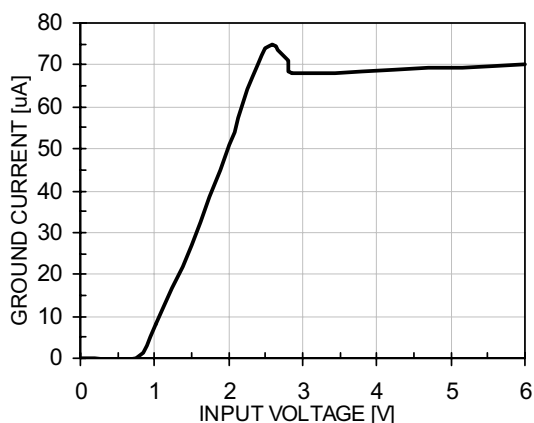
Ground Current vs. Input (5mA Load)
