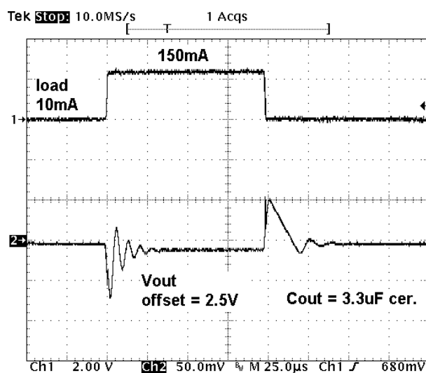
Figure 3. Stable Load Transient Response 2.5V output with 3.3 \mu F ceramic capacitor
