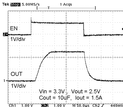
Enable Power-Up with 1.5A Load
