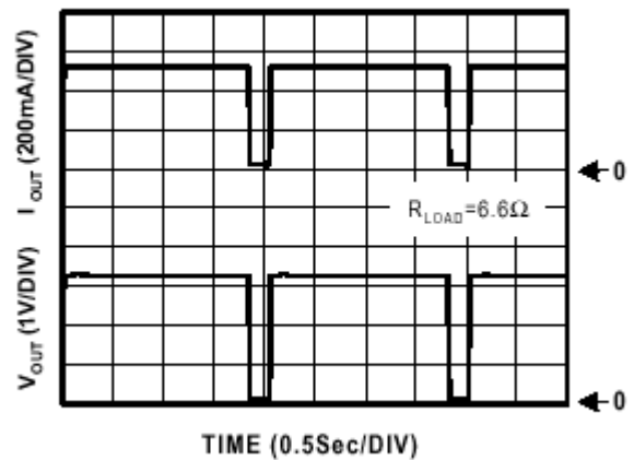
Overtemperature Shutdown
