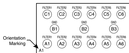
CM1450-06CS/CP 15-Bump CSP Package
