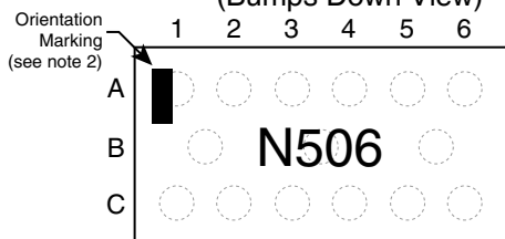
CM1450-06CS/CP 15-Bump CSP Package
