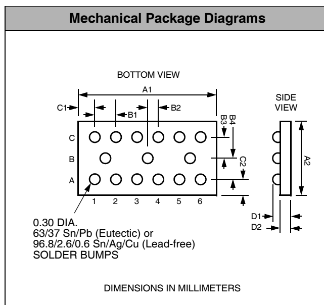
Package Dimensions for CM1450-06CS/CP Chip Scale Package
