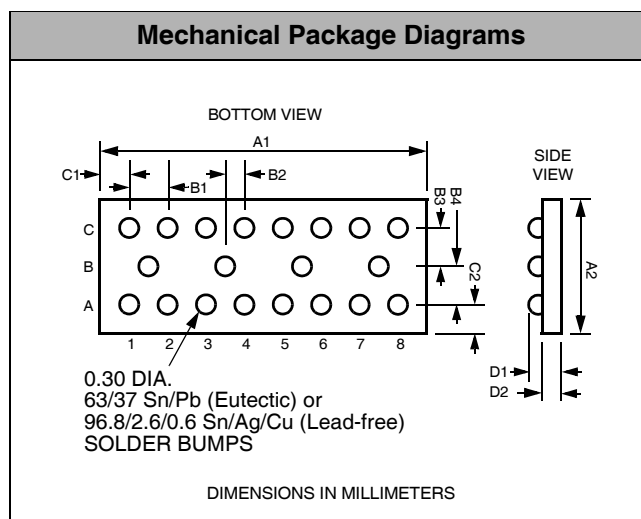
Package Dimensions for CM1450-08CS/CP Chip Scale Package
