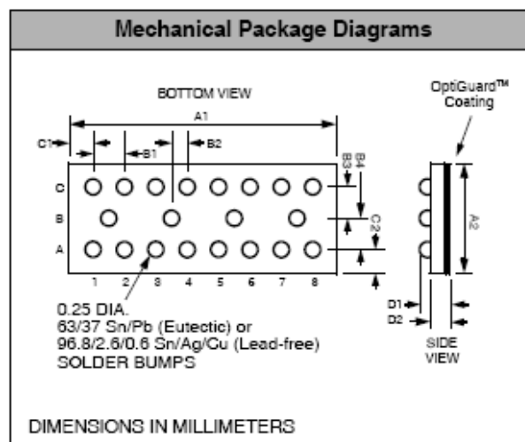
Package Dimensions for CM1442-08 Chip Scale Package
