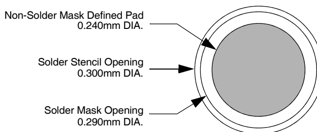
Figure 8. Recommended Non-Solder Mask Defined Pad Illustration
