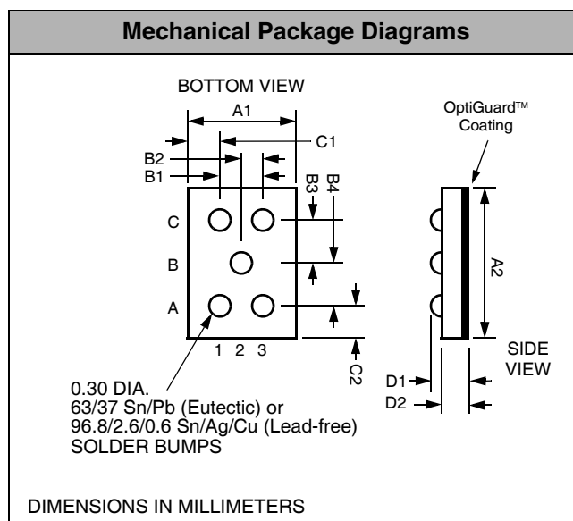
Package Dimensions for CM1414 Chip Scale Package
