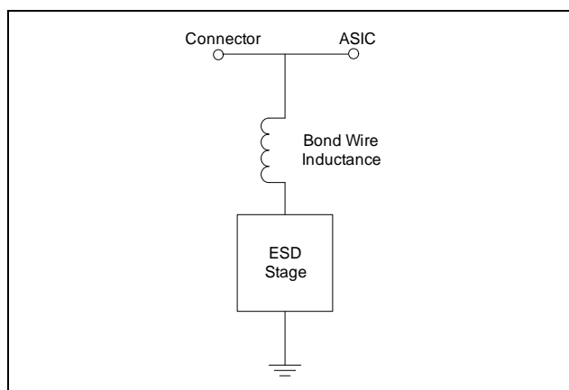
Figure 4. Single Stage ESD Protection Model
