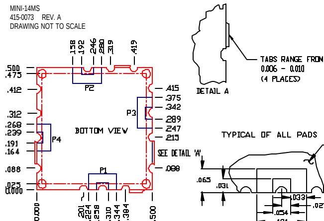
PHYSICAL DIMENSIONS
