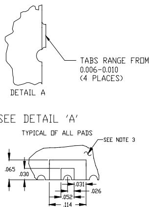
PHYSICAL DIMENSIONS
