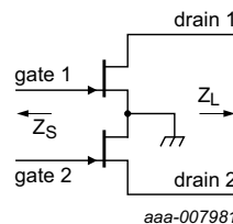
Fig 9. Definition of transistor impedance
