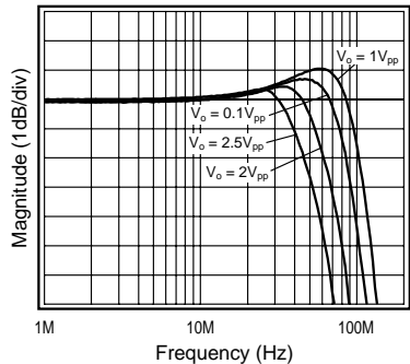
Gain Flatness
