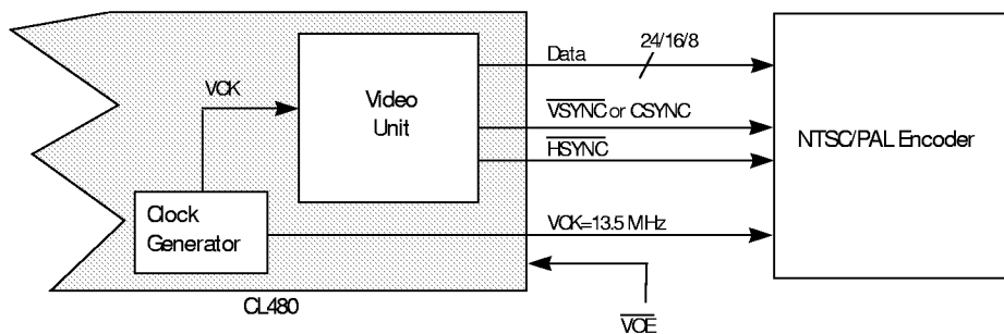
Figure 7-2 \overline{\text{VSYNC}} / \overline{\text{HSYNC}} /VCK Out Mode
