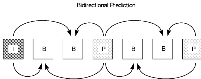
Figure 2-7 Bidirectional Prediction
