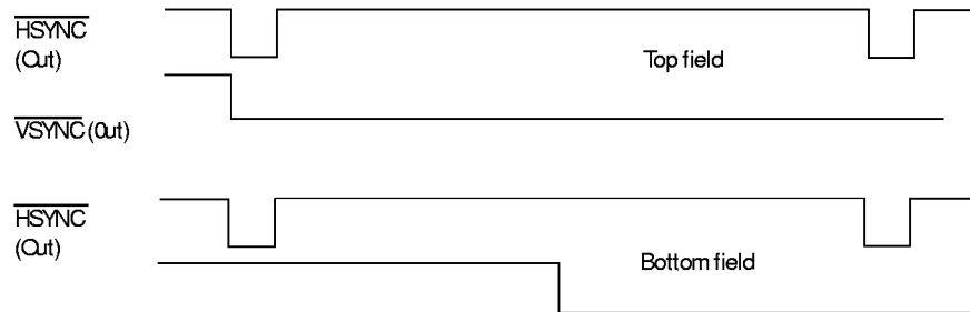
Figure 9-16 \overline{\text{VSYNC}} and \overline{\text{HSYNC}} Out
