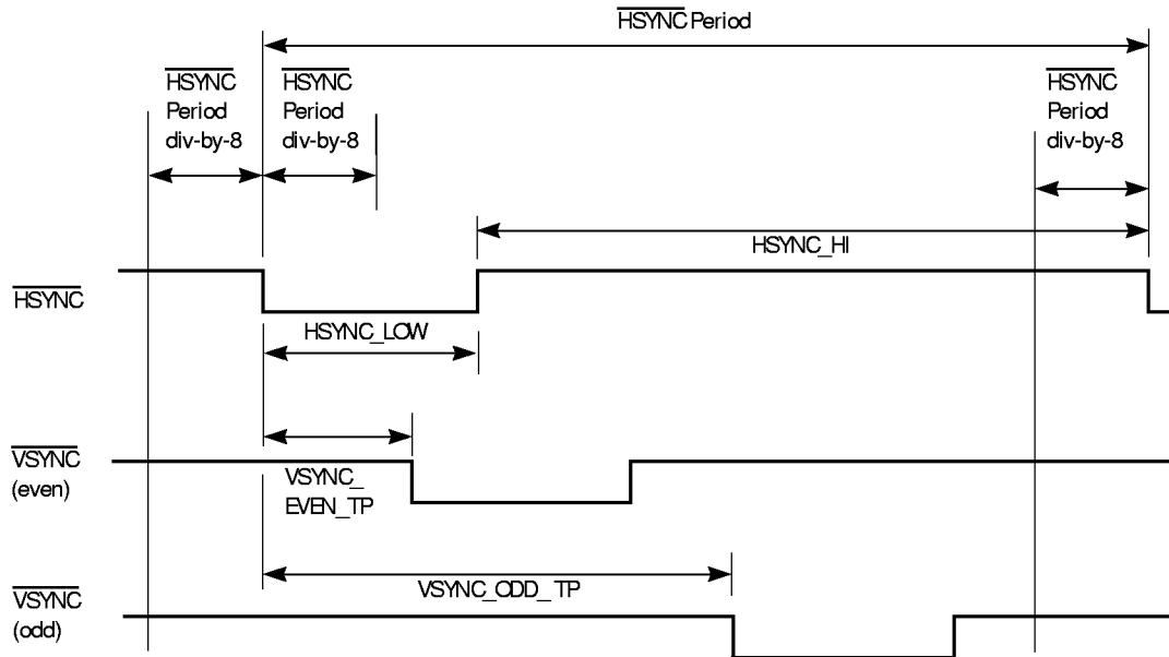
Figure 7-5 \overline{\text{HSYNC}} and \overline{\text{VSYNC}} Timing
