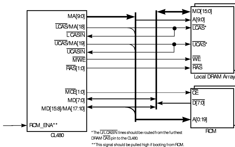
Figure 5-1 DRAM Interface
