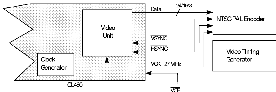
Figure 7-3 \overline{\text{VSYNC}} / \overline{\text{HSYNC}} /VCK In
