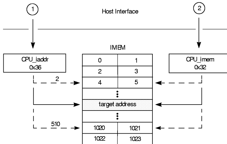
Figure 10-1 IMEM Write Data Flow
