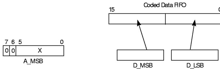
Figure 4-5 CFIFO Register Address Formed by A_MSB
