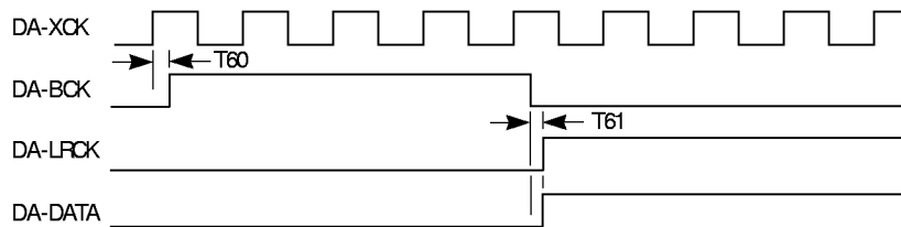
Figure 9-24 Audio Interface Timing Modes
