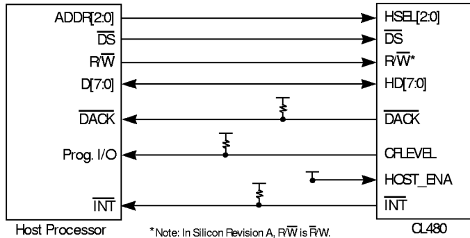
Figure 3-3 Host Interface Signals
