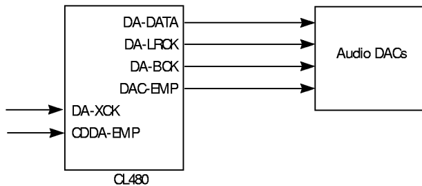
Figure 3-7 Audio Interface Signals
