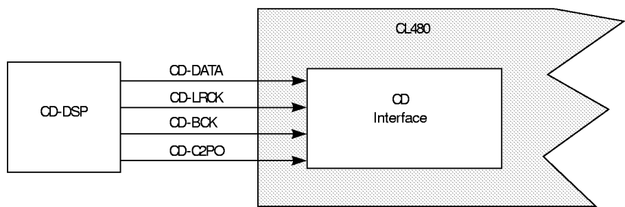
Figure 6-1 CD-Decoder Interface
