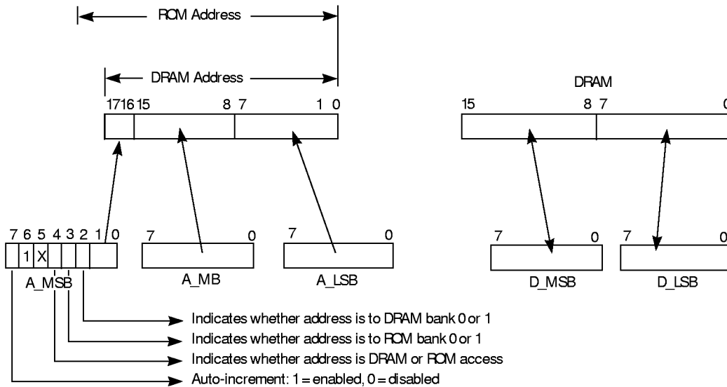
Figure 4-2 DRAM/ROM Address Formed by Host Address Registers
