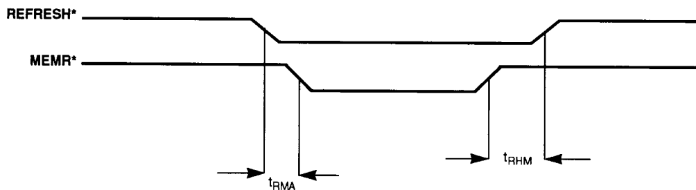
Figure 6-9. REFRESH* Timing (ISA Bus)
