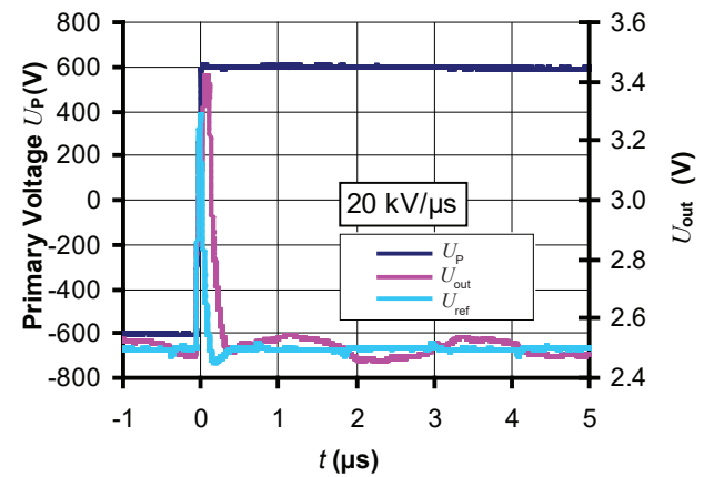
Figure 6: du/dt
