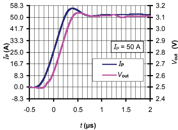
Figure 21: Step response
