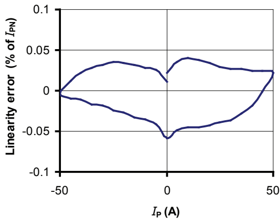
Figure 19: Linearity error
