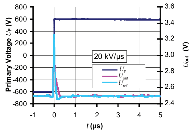
Figure 24: du/dt
