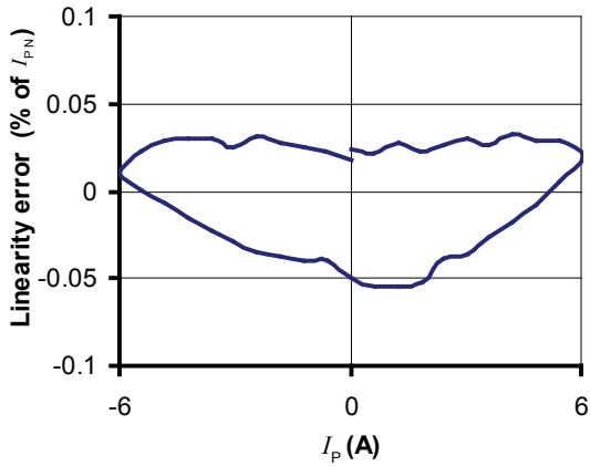
Figure 1: Linearity error
