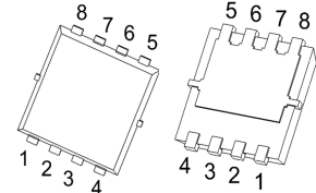
PDFNWB3.3×3.3-8L
