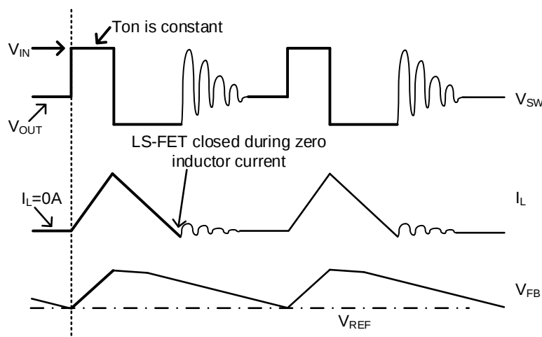
Figure 8-3 PFM Operation
