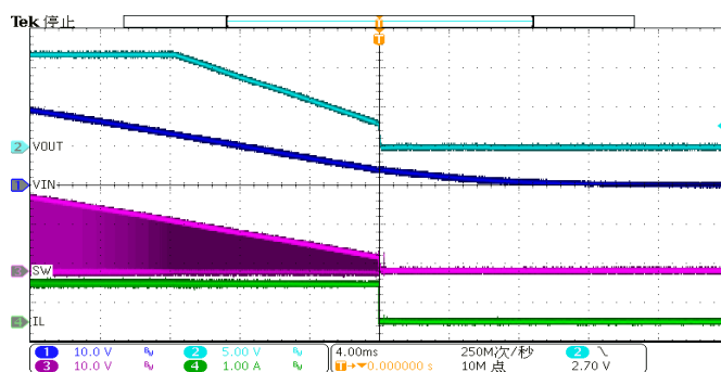
Shut Down through V_{IN} ( I_{OUT} = 1A )
