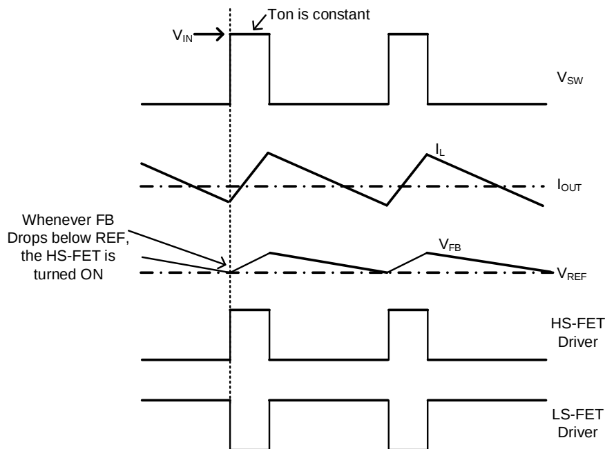
Figure 8-2 FPWM Operation
