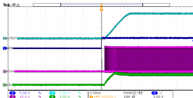
Start-Up through EN ( I_{OUT} = 1A )
