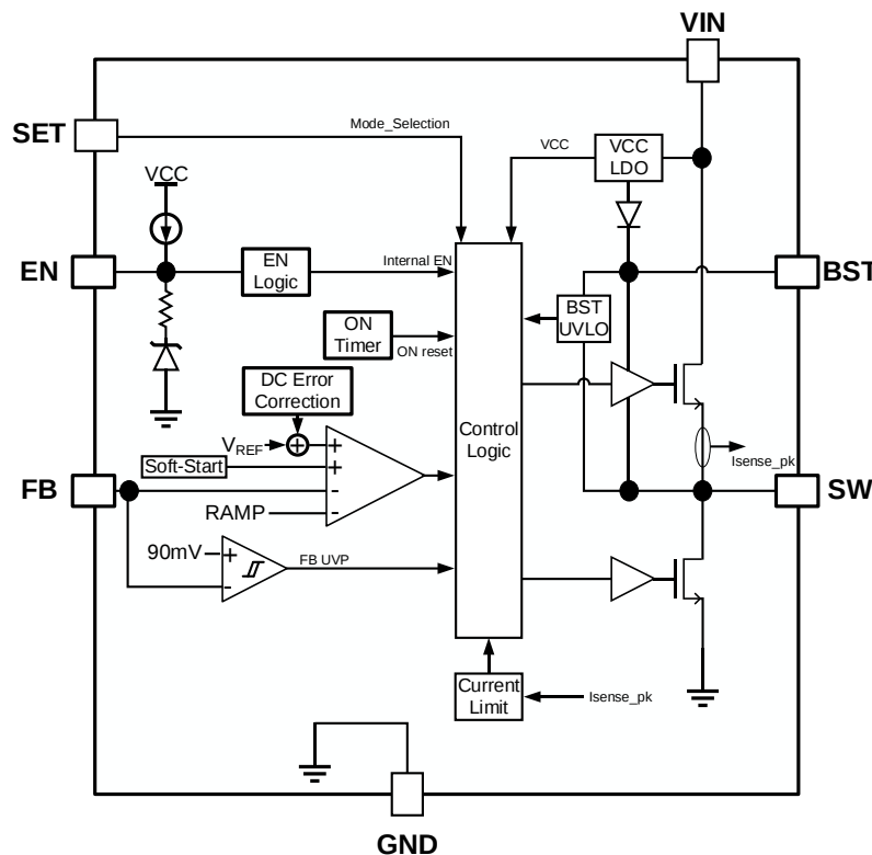
Figure 8-1 Function block diagram
