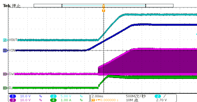
Start-Up through V_{IN} ( I_{OUT} = 1A )
