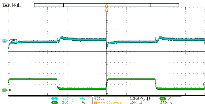
Load Transient
