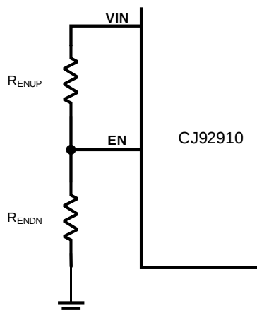
Figure 8-4 EN network
