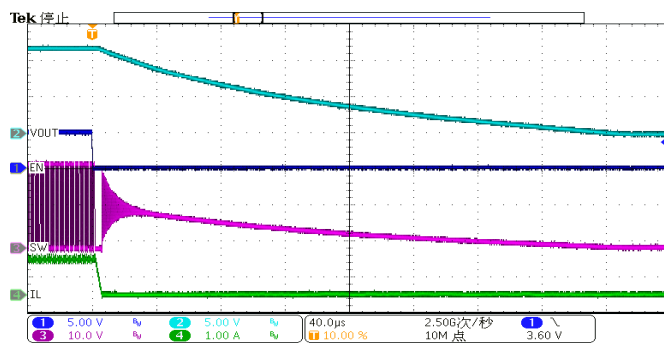
Shut-Down through EN ( I_{OUT}=1A )
