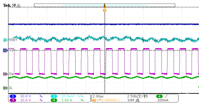
Output Voltage Ripple ( I_{OUT} = 1A )
