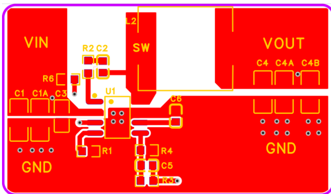
Figure 10-1. Top Layer
