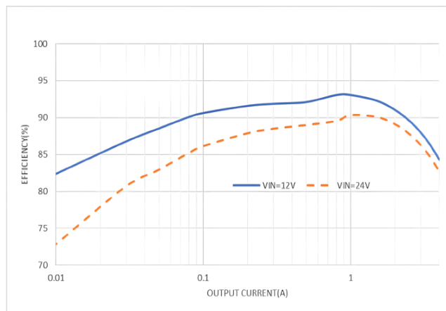
Efficiency vs. Load Current, L=6.8\mu H , DCR= 48mohm V_{OUT}=3.3V
