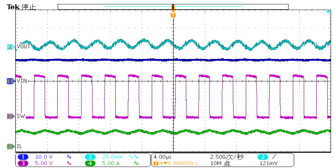
Output Voltage ripple (IOUT=4A)
