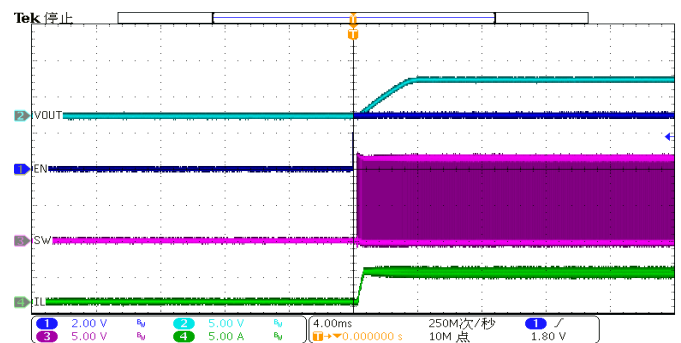
Start – Up through EN (IOUT=4A)
