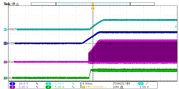
Start – Up through VIN (IOUT=4A)
