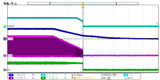
Shutdown through VIN (IOUT=4A)
