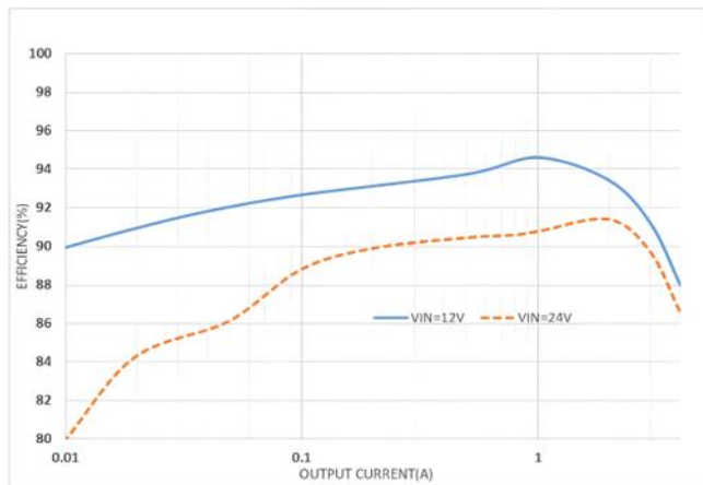
Efficiency vs. Load Current, L=6.8\mu H , DCR= 48mohm V_{OUT}=5V
