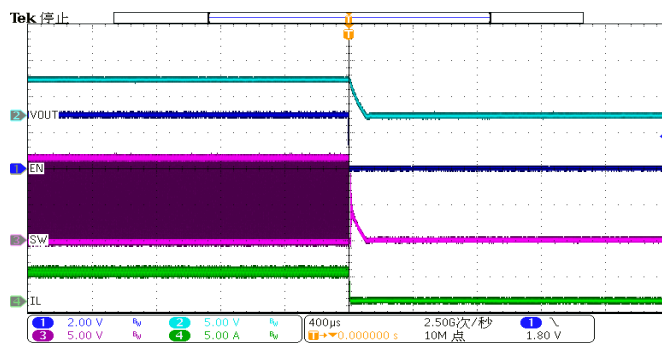
Shutdown through EN (IOUT=4A)
