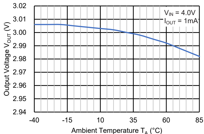
3.0V Output Temperature Characteristics
