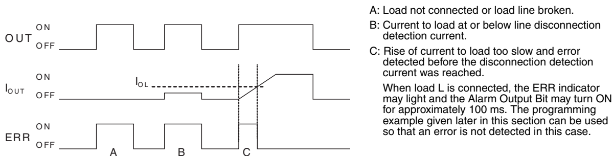
Figure 3: Line Disconnections
