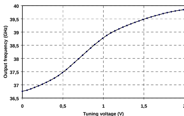
Typical tuning characteristic
