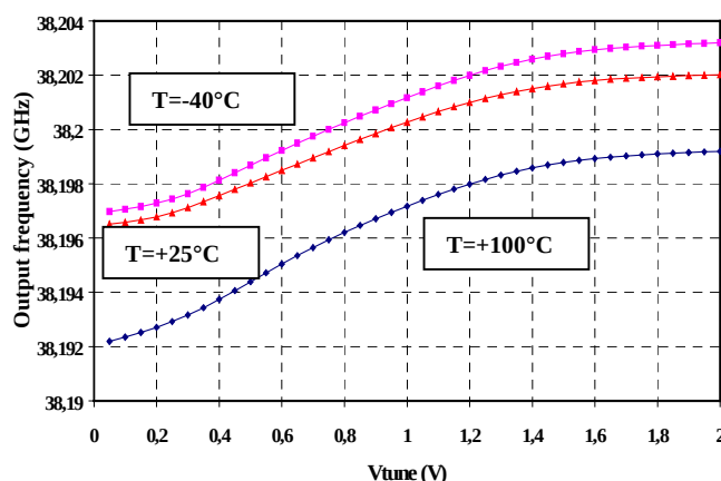
Typical tuning characteristic
