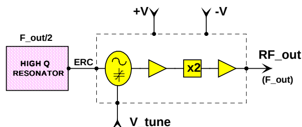
Multifunction block diagram
