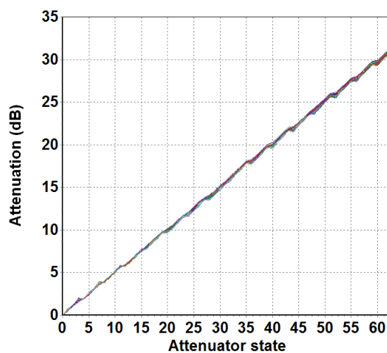
Attenuation versus attenuator state Frequency bandwidth 4-14GHz
