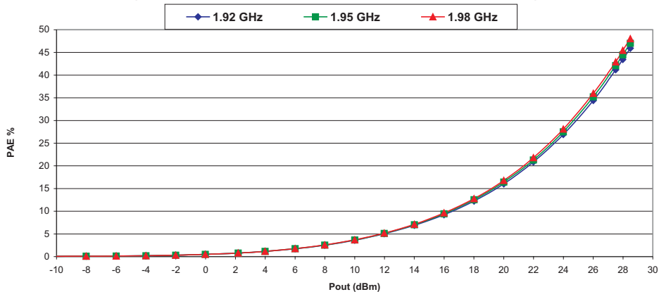
Figure 6: PAE vs P_{OUT} (T = +25 °C, V_{CC} = 3.4 V, V_{REF} = 2.85 V, V_{MODE} = 2.85 V) www.DataSheet4U.com
