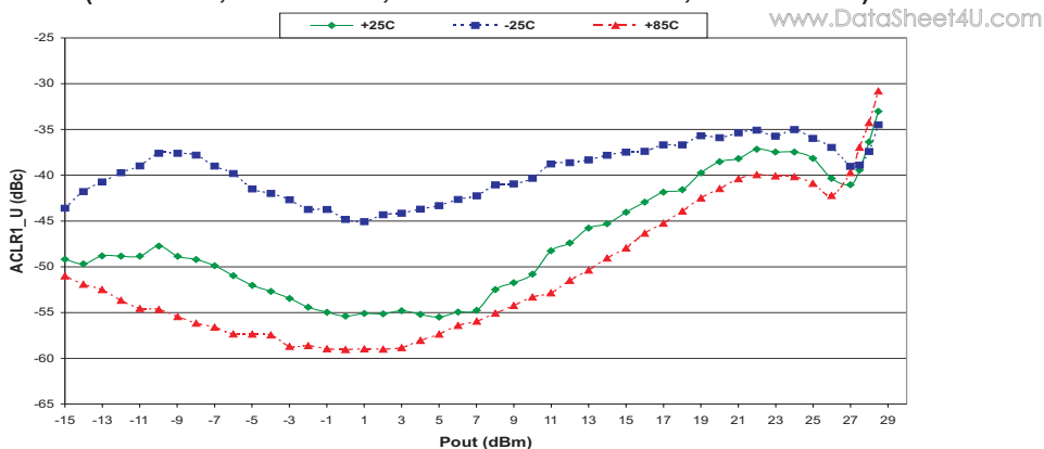
Figure 21: ACLR1_U vs Po (V_{CC} = 3.4 \text{ V}, V_{REF} = 2.85 \text{ V}, V_{MODE} = 1.5 + 0.025 \cdot P_{OUT}, F = 1.95 \text{ GHz})
